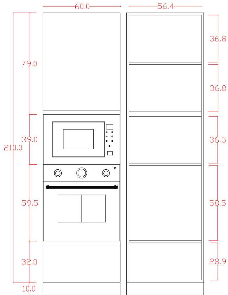
HIGH CABINET FRONT VIEW
