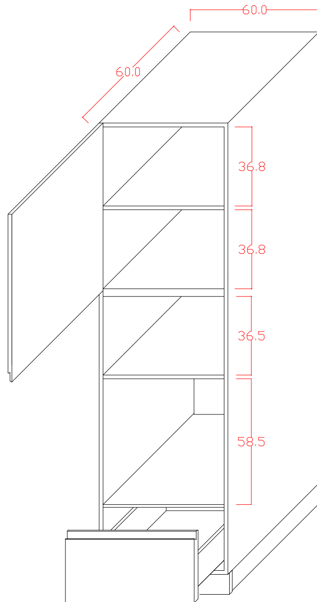
HIGH CABINET PERSPECTIVE
