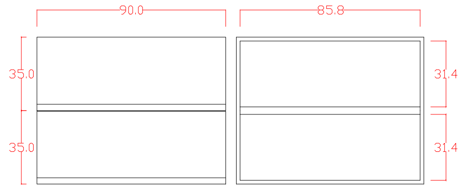
WALL CABINET FRONT VIEW
