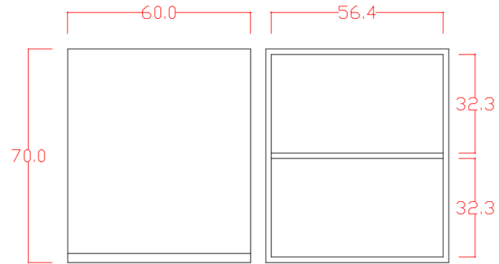
WALL CABINET FRONT VIEW
