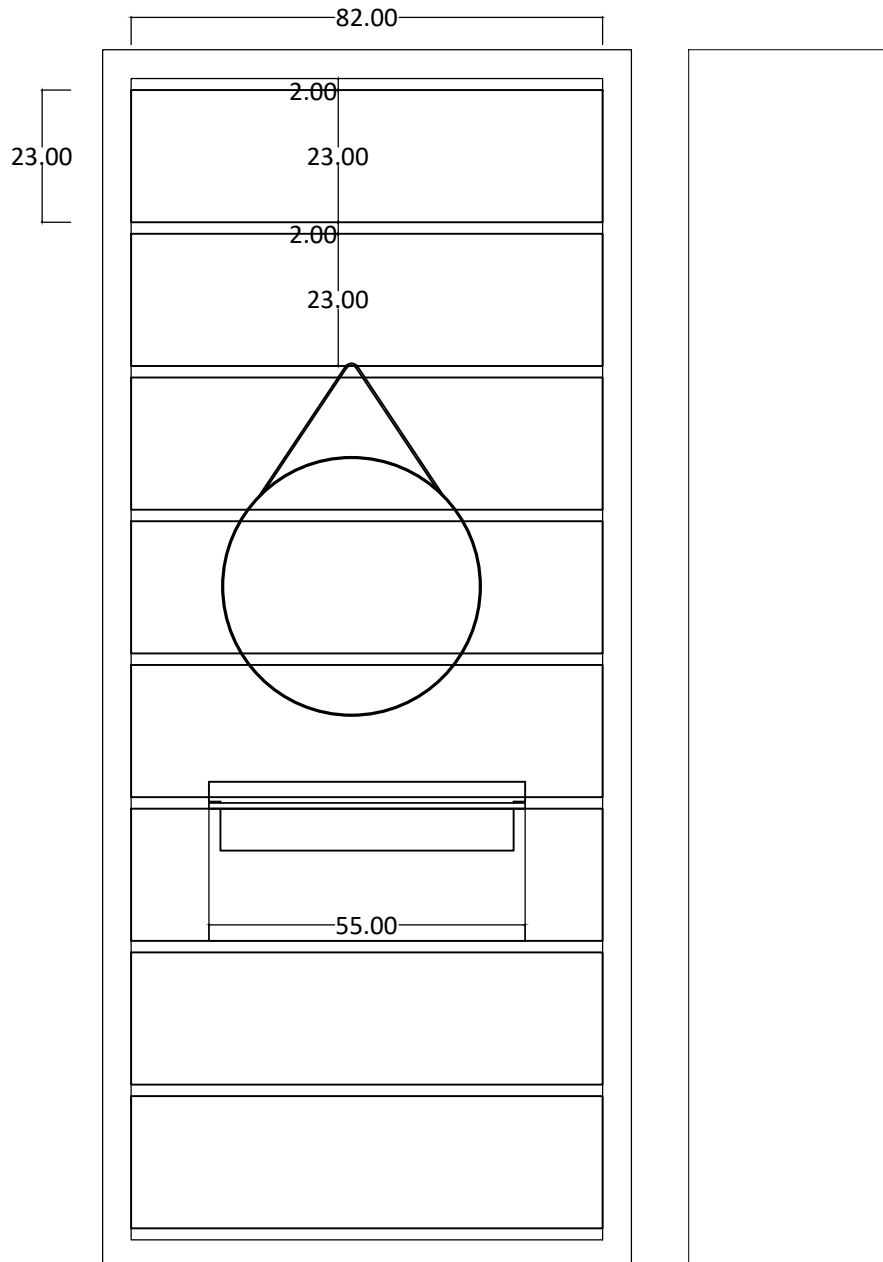
FRONT VIEW (WOOD IS INCLUDING)
