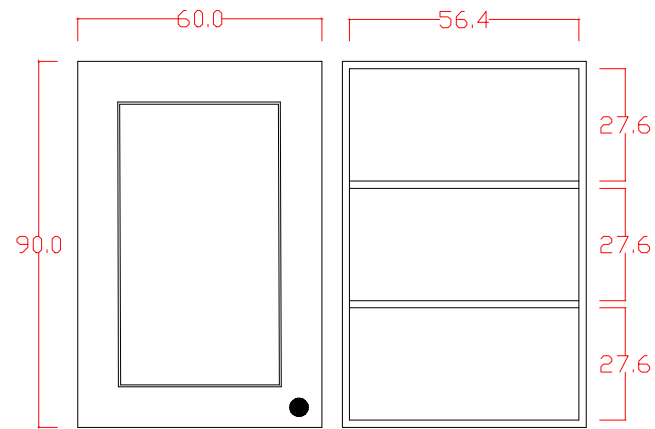
WALL CABINET FRONT VIEW
