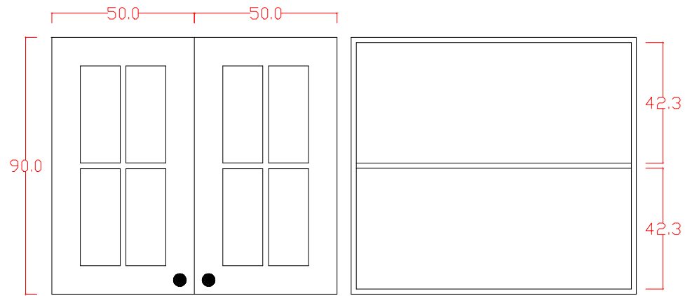
WALL CABINET FRONT VIEW
