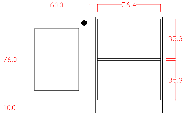
BASE CABINET FRONT VIEW
