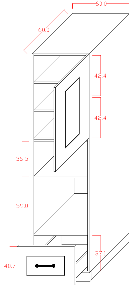
HIGH CABINET PERSPECTIVE
