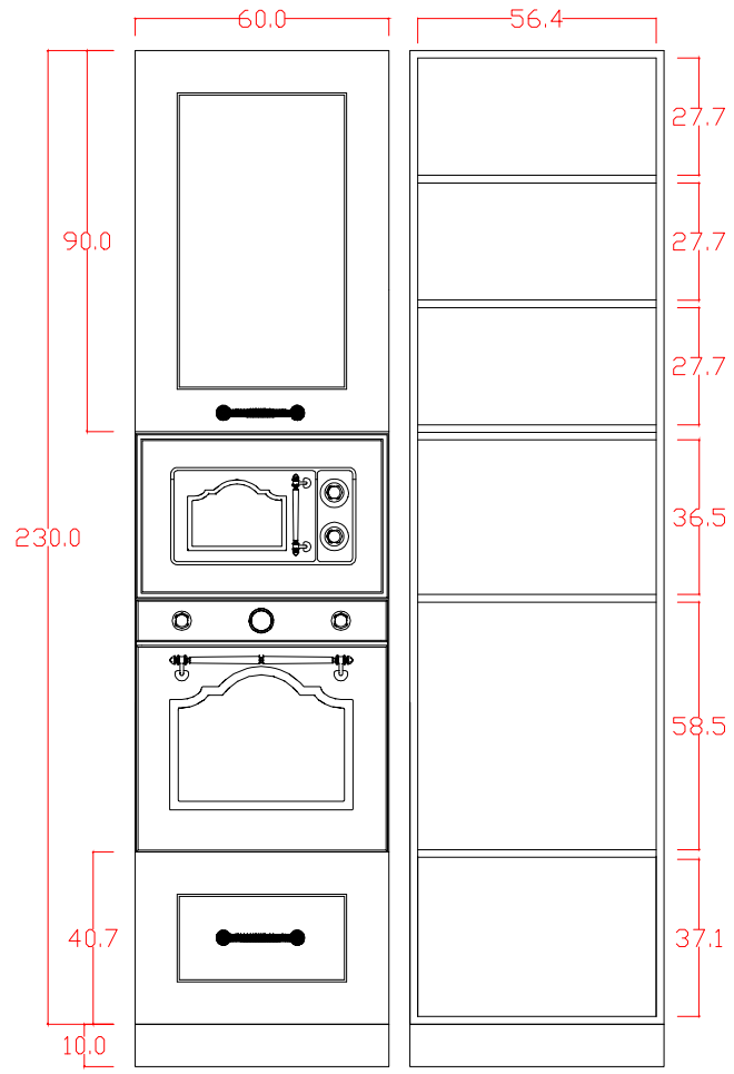
HIGH CABINET FRONT VIEW
