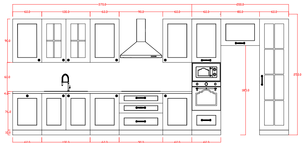
KITCHEN 2 FRONT VIEW
