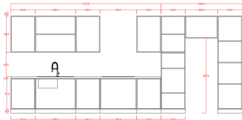
KITCHEN 2 FRONT VIEW
