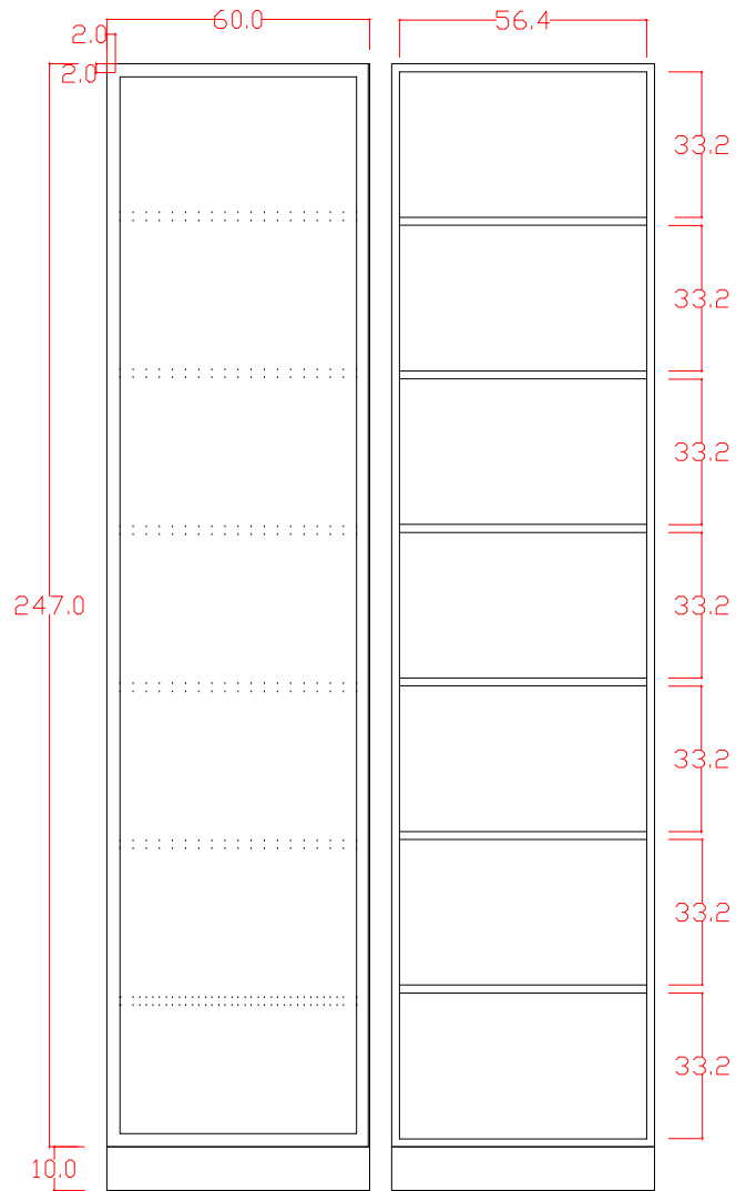
HIGH CABINET FRONT VIEW
