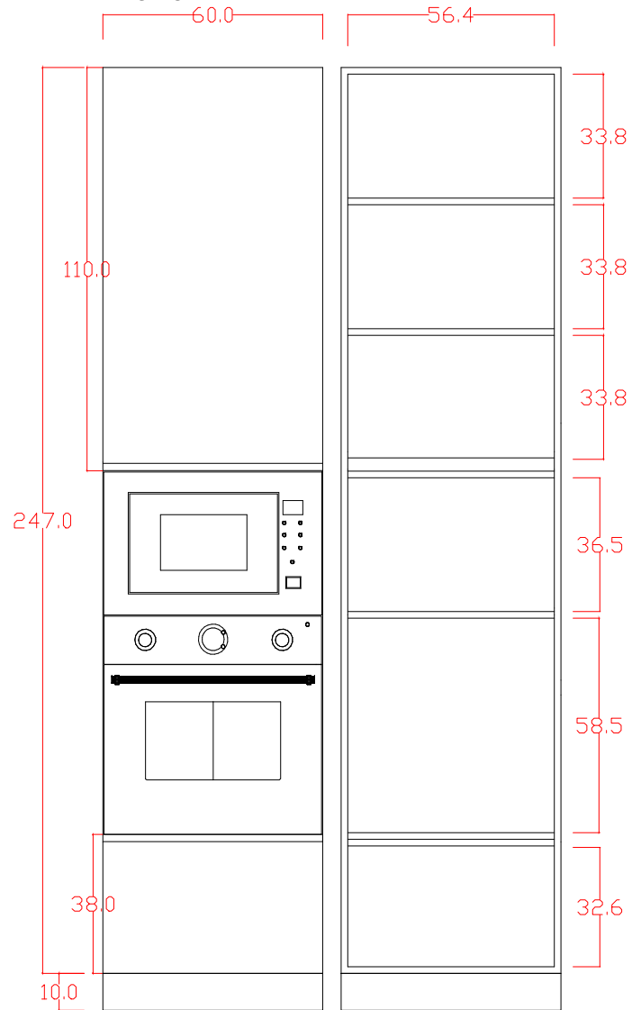
HIGH CABINET FRONT VIEW
