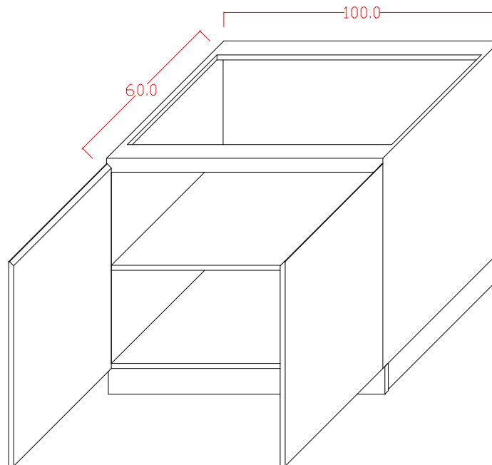
BASE CABINET PERSPECTIVE
