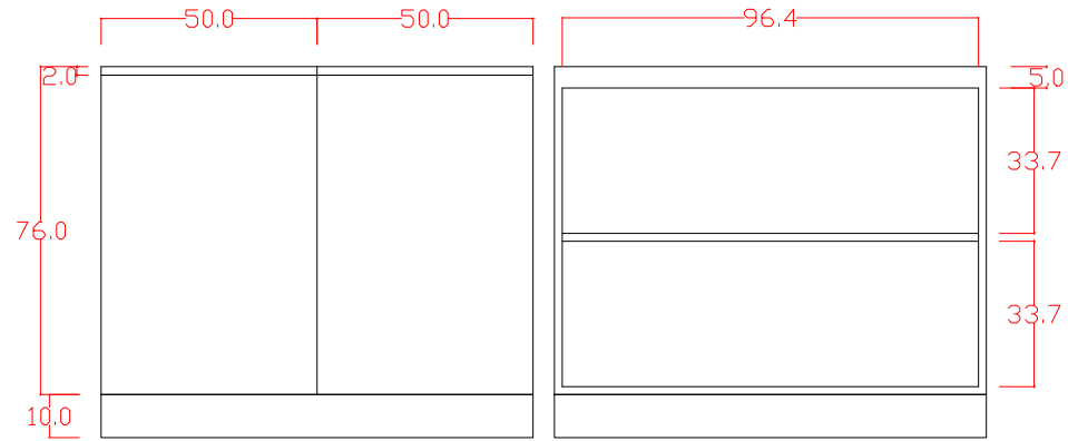
BASE CABINET FRONT VIEW
