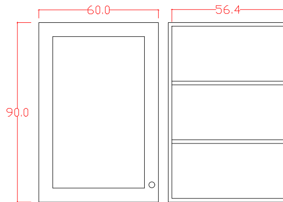
WALL CABINET FRONT VIEW
