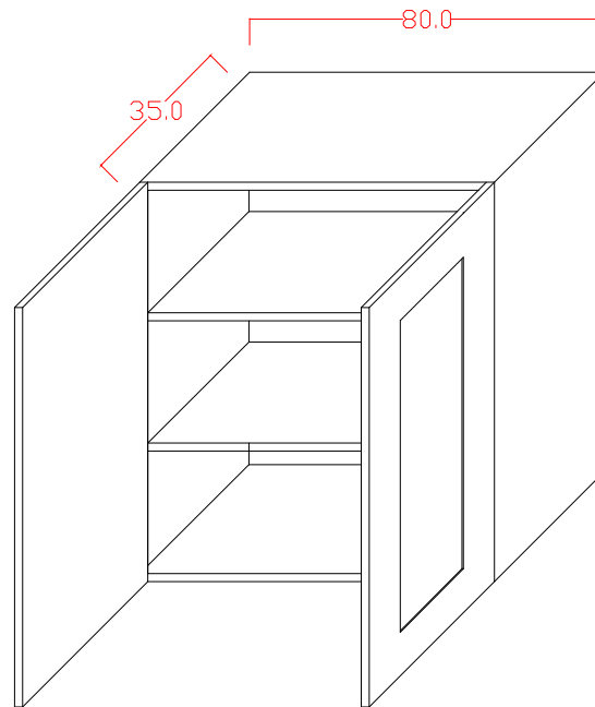
WALL CABINET PERSPECTIVE
