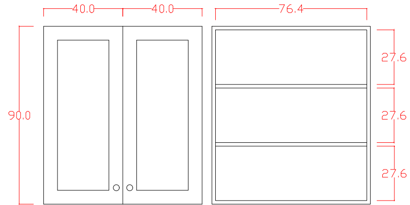
WALL CABINET FRONT VIEW
