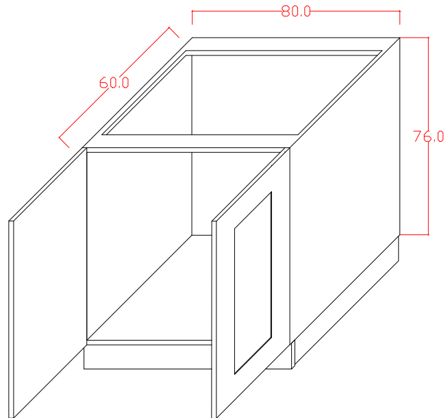
BASE CABINET PERSPECTIVE
