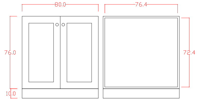
BASE CABINET FRONT VIEW
