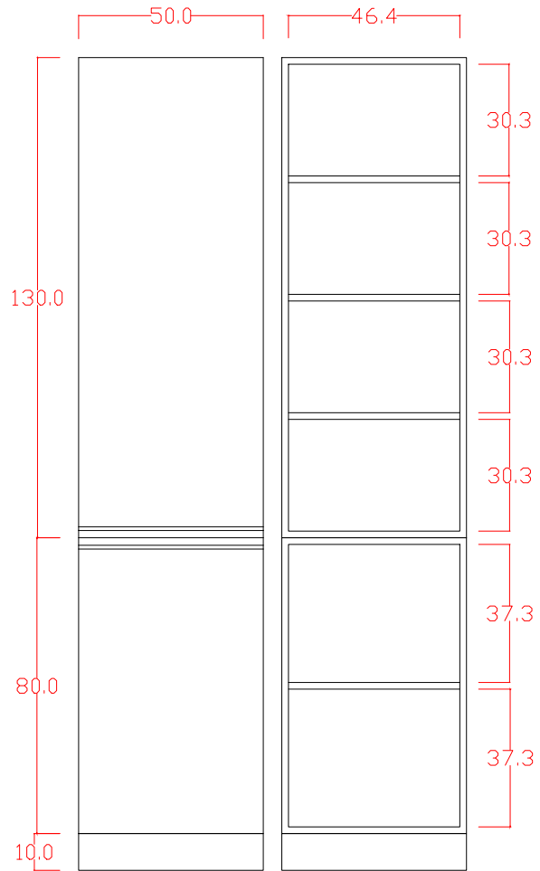
HIGH CABINET FRONT VIEW
