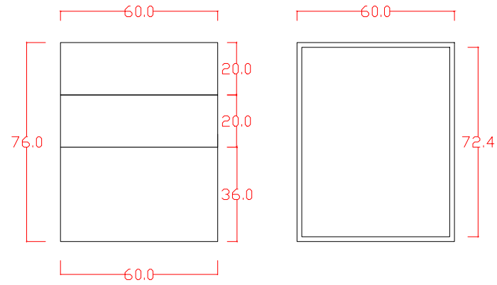
BASE CABINET FRONT VIEW
