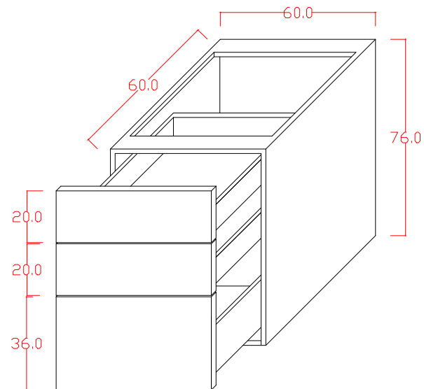
BASE CABINET PERSPECTIVE
