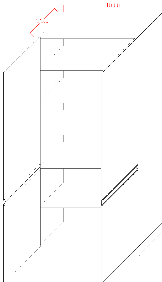
HIGH CABINET PERSPECTIVE
