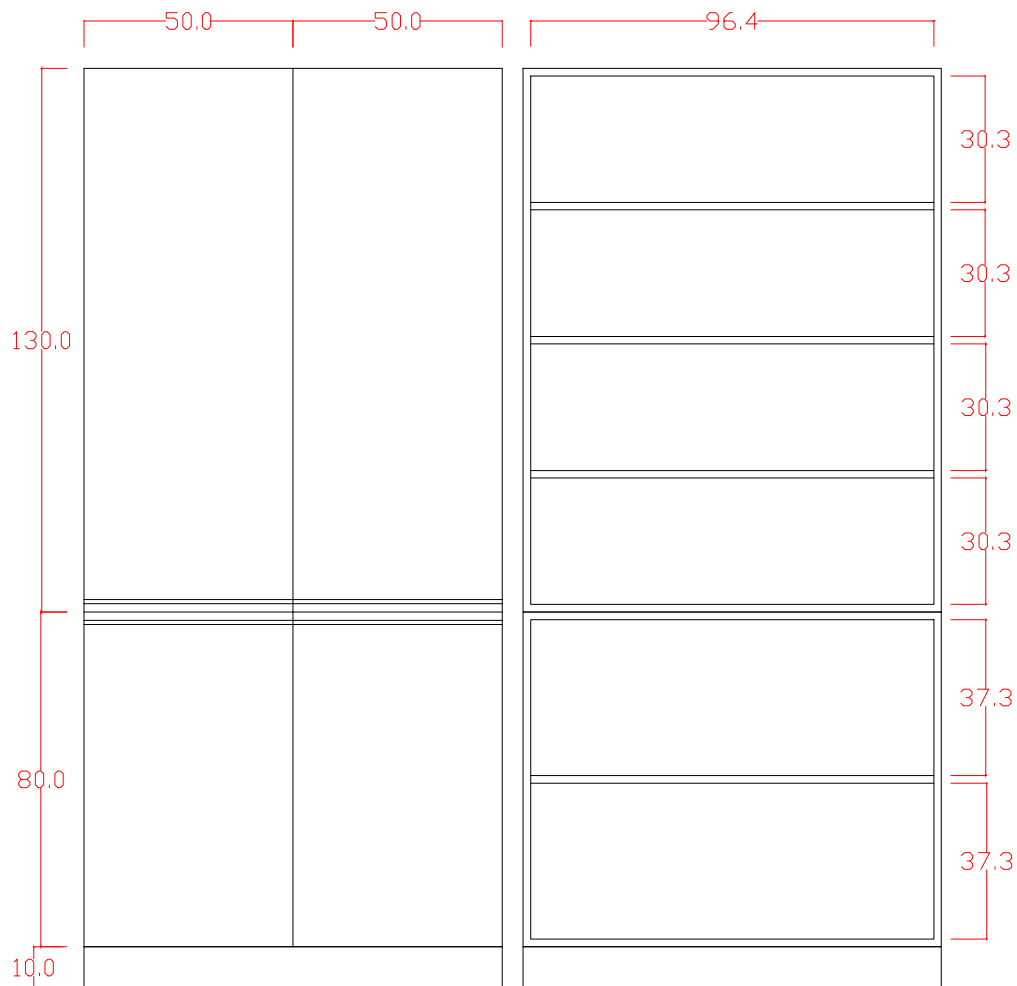
HIGH CABINET FRONT VIEW
