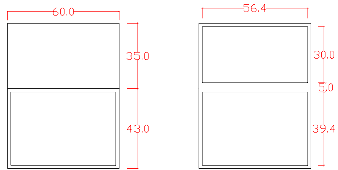
BASE CABINET FRONT VIEW
