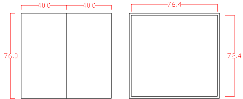
BASE CABINET FRONT VIEW
