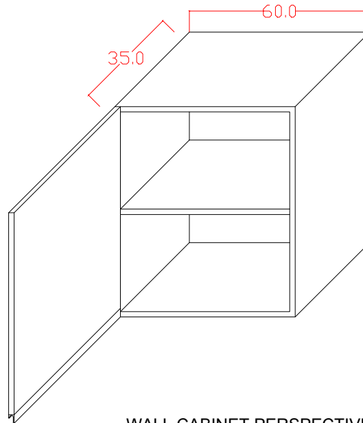
WALL CABINET PERSPECTIVE
