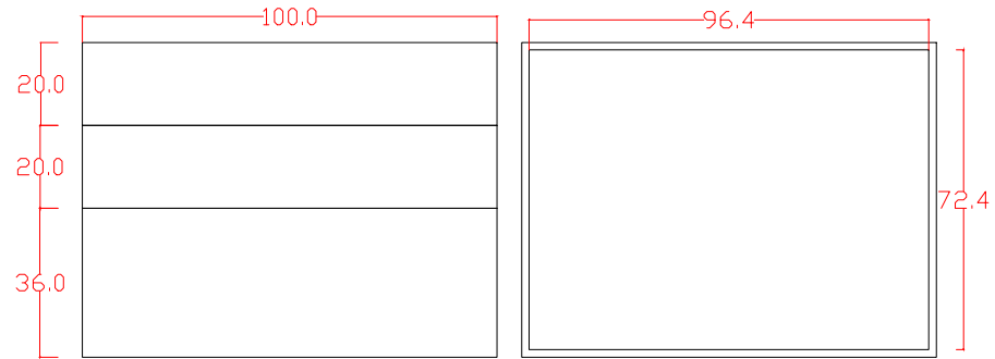
BASE CABINET FRONT VIEW
