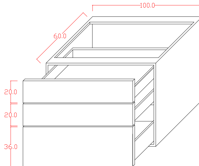
BASE CABINET PERSPECTIVE
