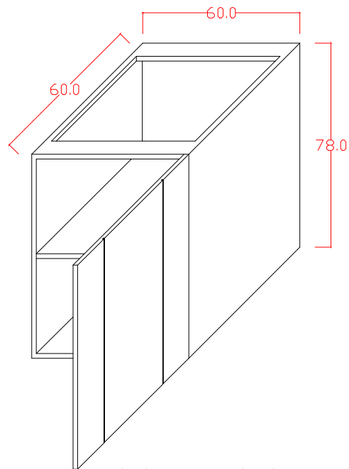
BASE CABINET PERSPECTIVE
