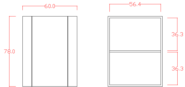
BASE CABINET FRONT VIEW
