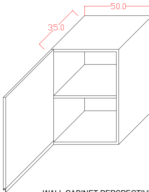
WALL CABINET PERSPECTIVE
