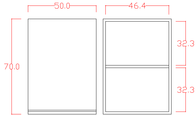
WALL CABINET FRONT VIEW
