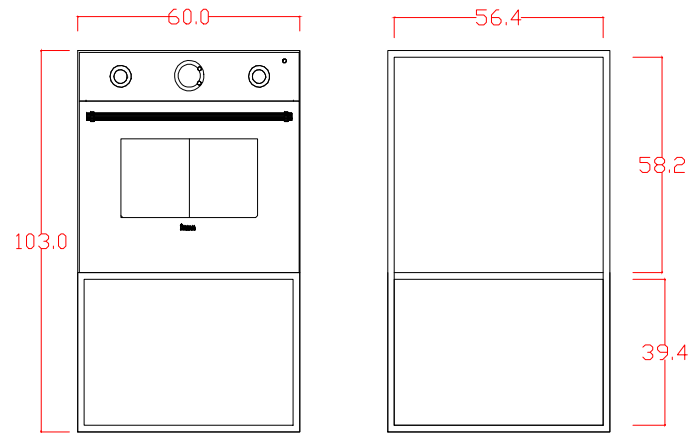
BASE CABINET FRONT VIEW
