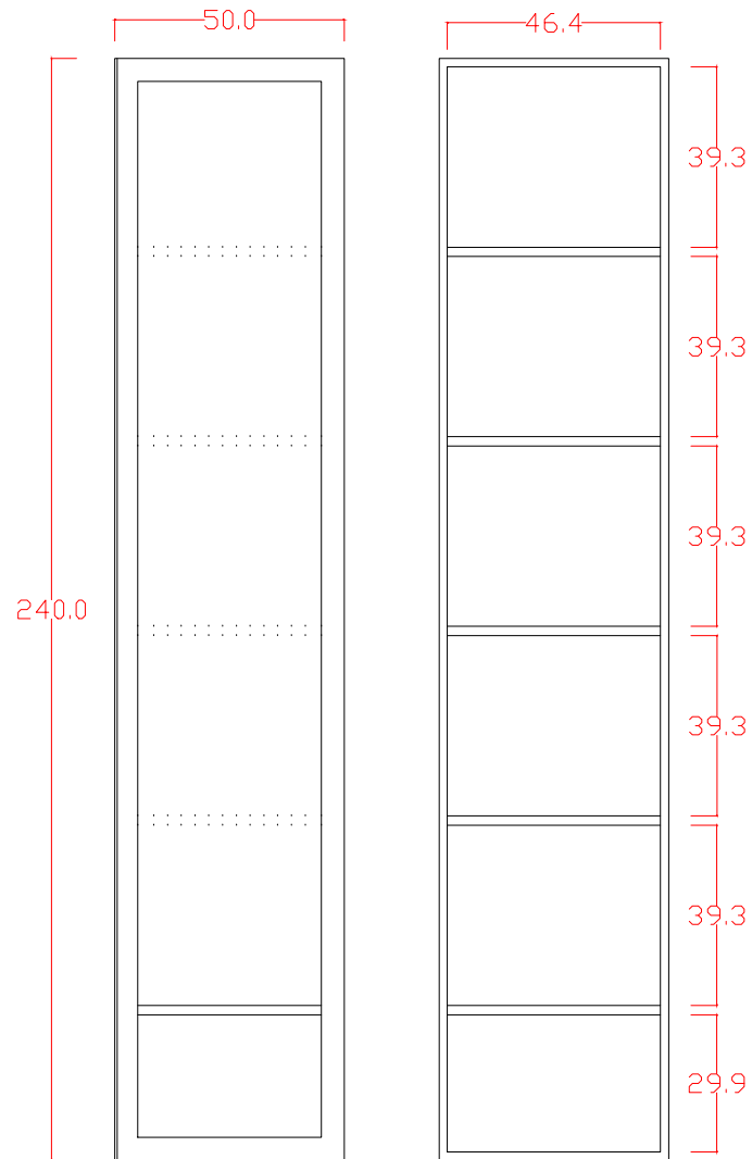
HIGH CABINET FRONT VIEW
