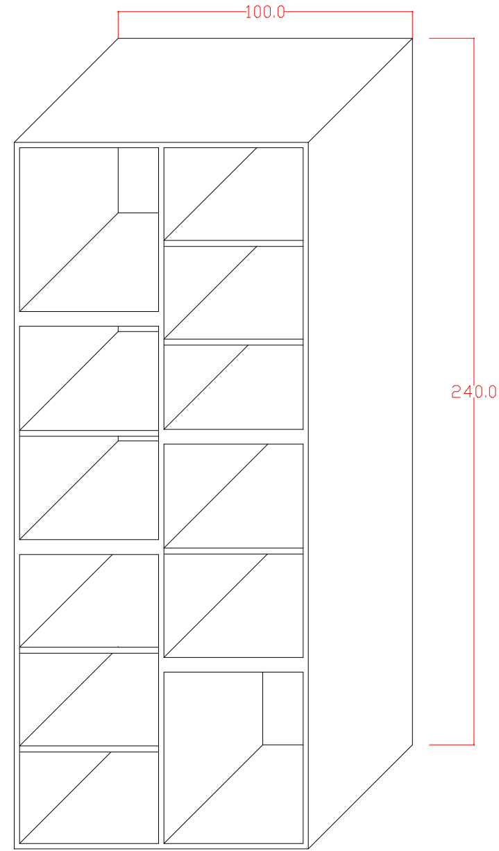
HIGH CABINET PERSPECTIVE
