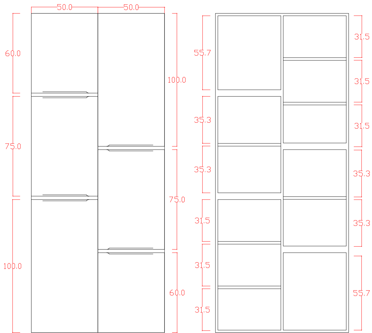
HIGH CABINET FRONT VIEW
