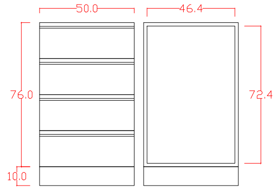
BASE CABINET FRONT VIEW
