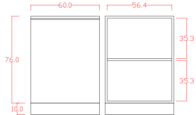
BASE CABINET FRONT VIEW
