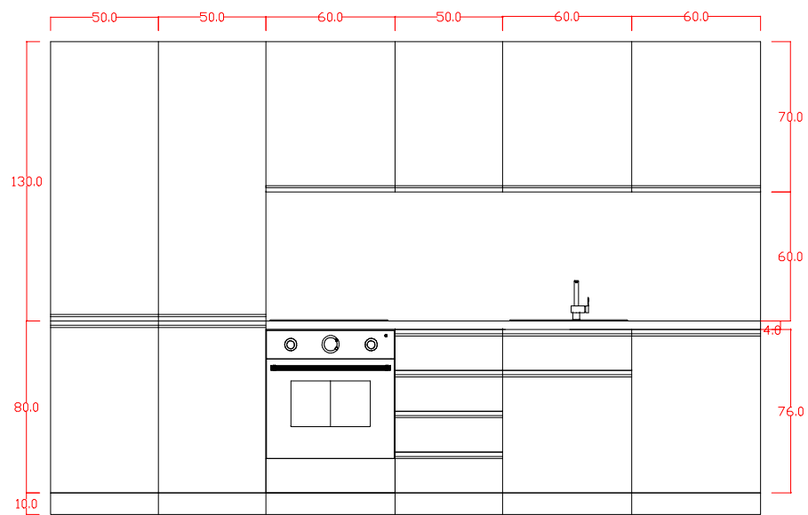
KITCHEN 6 FRONT VIEW
