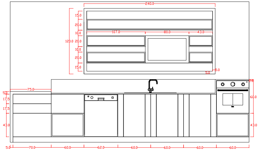
KITCHEN 5 FRONT VIEW
