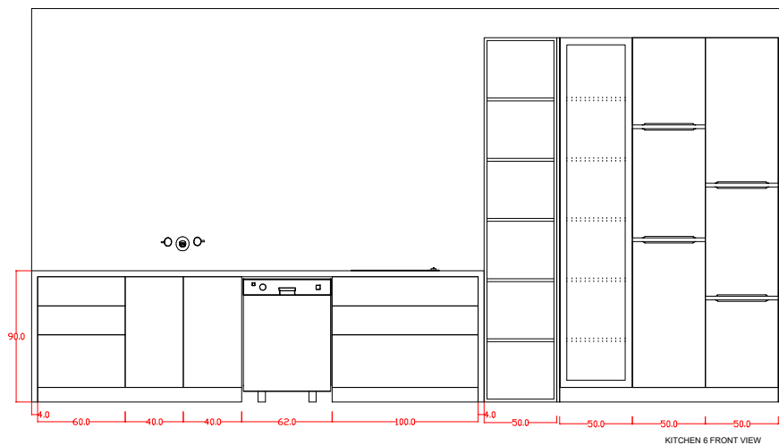
KITCHEN 6 FRONT VIEW
